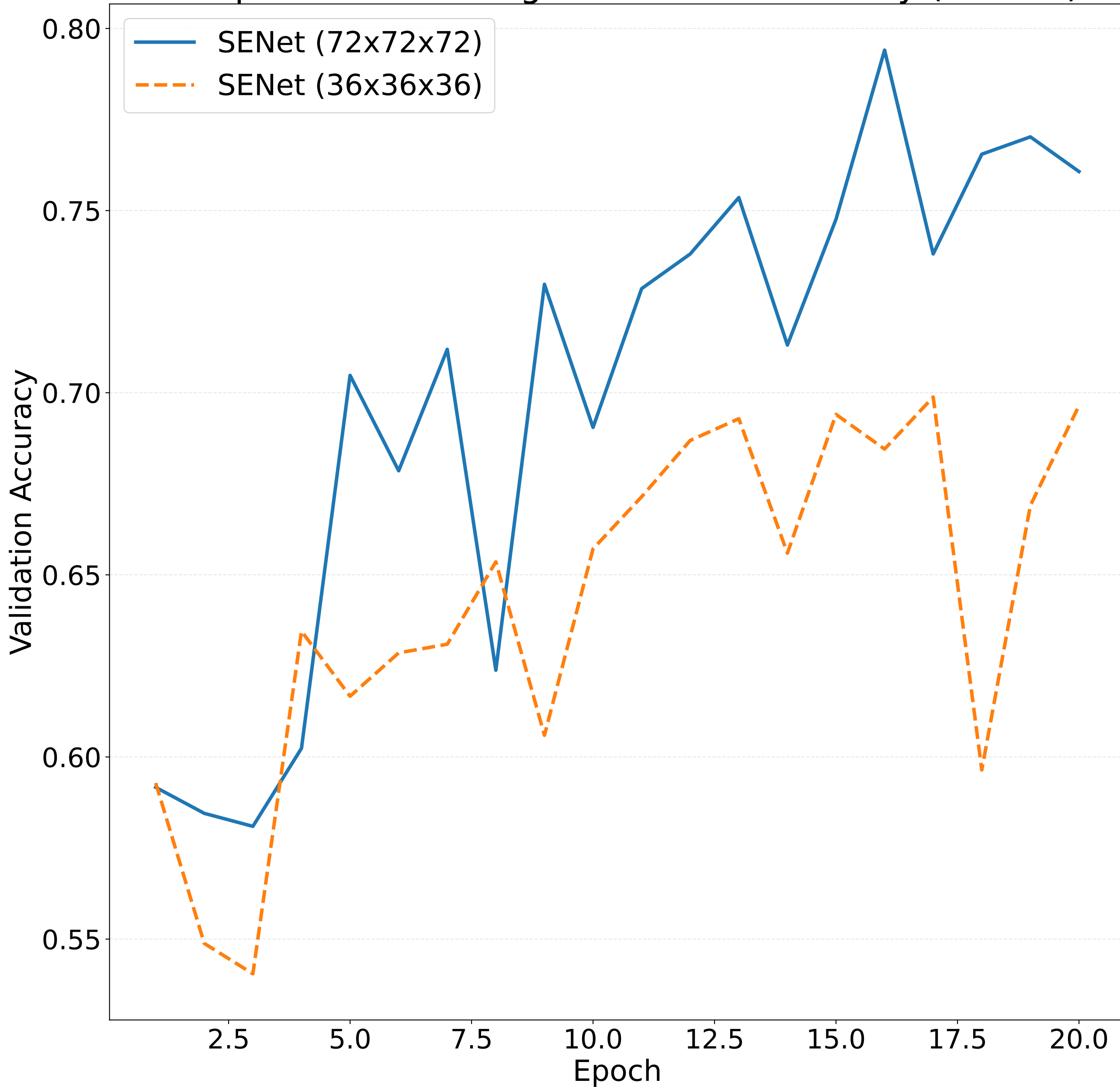
Comparison of Average Validation Accuracy (5 Folds)
